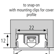
cover profile for milled groove
