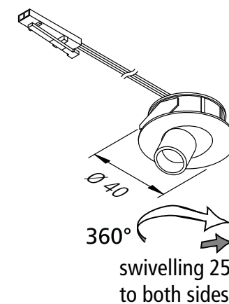
LED Eye 25S
