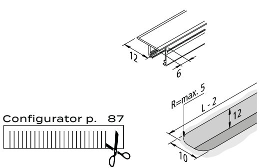
MILLED PROFILE 12MM
