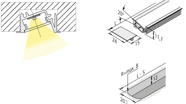
MILLED PROFILE I 24MM
