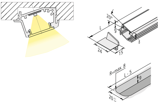
MILLED PROFILE A 24MM
